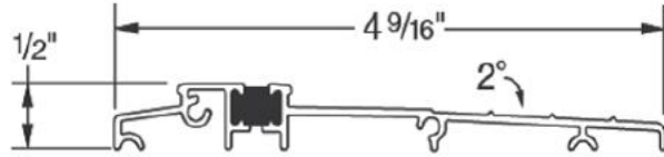
PART # HC4562
