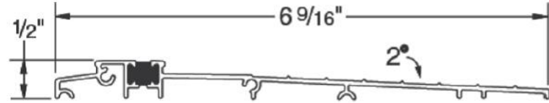
PART # HC6562
