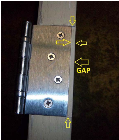
4" x 4" Hinge on Fiberglass Door. Note the "GAP".
